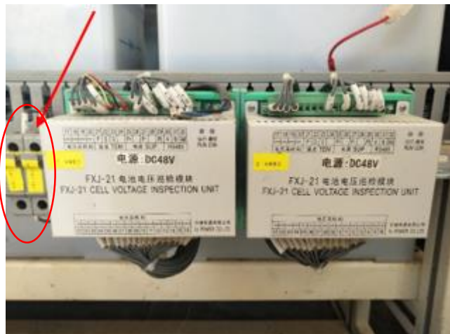
Figure 5: Porte-fusibles
